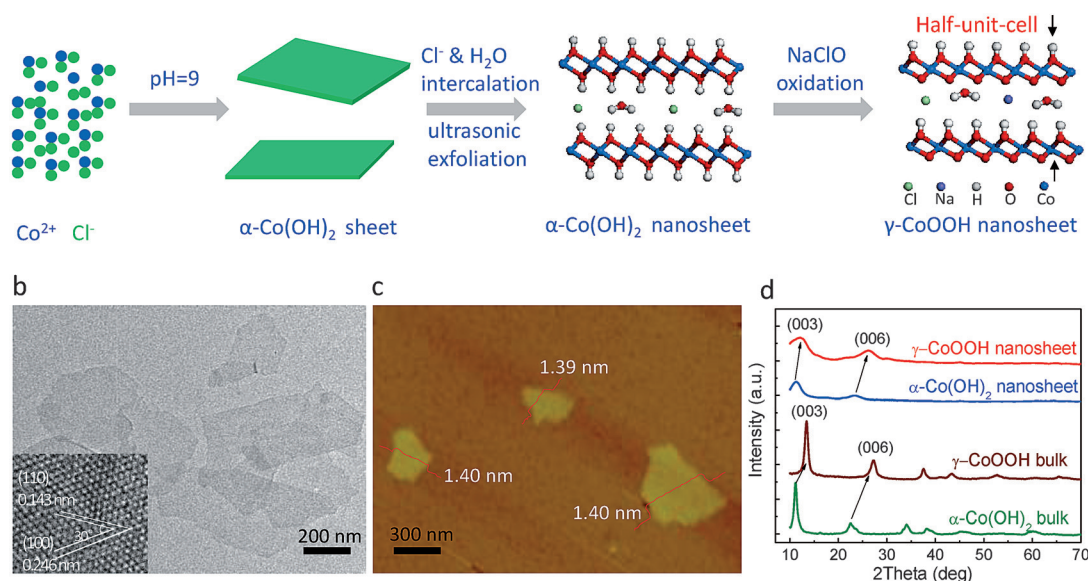
Figure 1. a) Synthetic route for the \gamma -CoOOH nanosheets. b) TEM image and c) AFM image for the \gamma -CoOOH nanosheets. The inset in (b) shows the HRTEM image for the \gamma -CoOOH nanosheets. d) XRD pattern for the \gamma -CoOOH nanosheets. The patterns of bulk \gamma -CoOOH and bulk and nanosheet \alpha -Co(OH) 2 are also displayed for comparison.
